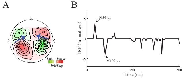
Figure 3: A) MEG magnetic field distribution for the first DSS component of a sample subject shows a stereotypical pattern of neural activity, originating separately in the left and right auditory cortices. Red and green contours represent the magnetic field strength. Blue arrows schematically represent the locations of the dipole currents, generating the measured magnetic field. B) Estimated TRF for the sample subject has significant components analogous to the well-known M50 and M100 auditory responses, as well as later responses, as demonstrated in the figure.
