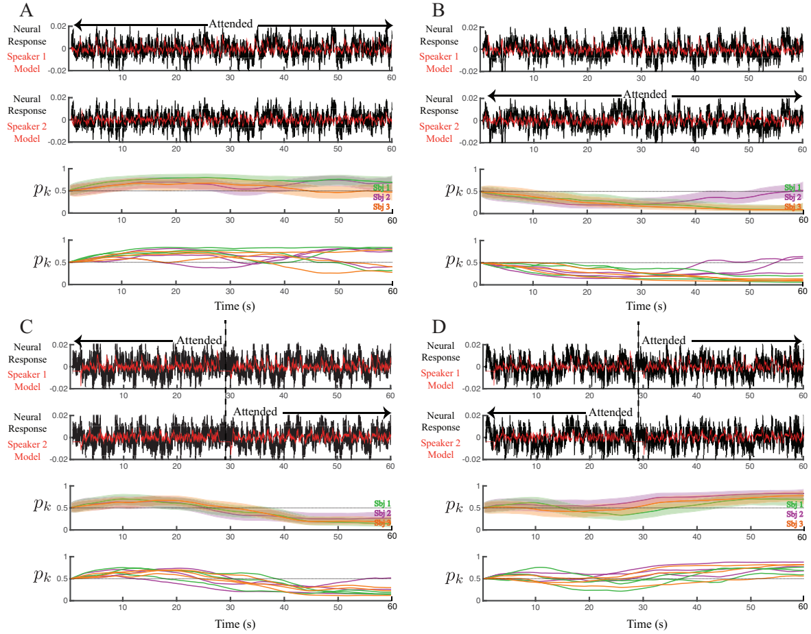
Figure 5: Decoding auditory attentional modulation in experimental MEG data. In each subplot, the neural response (black traces) and the model prediction (red traces) for attending to speaker one and speaker two are shown in the first and second panels, respectively, for one sample subject. The third panel shows the estimated values of \{p_k\} and the corresponding confidence intervals using multi-trial analysis for three sample subjects. The fourth panel shows the estimated \{p_k\} values for single trials. A) Condition 1: attending to the speaker one through the entire trial. B) Condition 2: attending to the speaker two through the entire trial. C) Condition 3: attending to the speaker one until t = 28s and switching attention to the speaker two after the 2 s pause. D) Condition 4: attending to the speaker two until t = 28s and switching attention to the speaker one after the 2 s pause. Dashed lines in subplots C and D indicate the start of the 2s silence cue for attentional switch. Error hulls indicate 90% confidence intervals. The MEG units are in pT/m .
