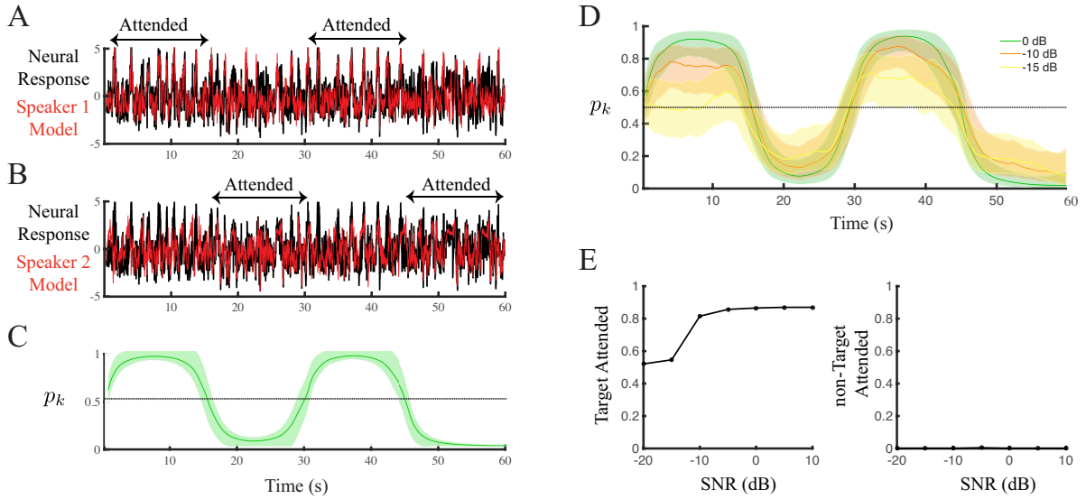
Figure 4: Simulated neural response (black traces) and model prediction (red traces) of A) speaker one and B) speaker two at SNR = 10 dB. Black arrows indicate the instructed attentional state of the subjects. The MEG units are in pT/m . C) Estimated values of \{p_k\} with 95% confidence intervals. D) Estimated values of \{p_k\} from simulated neural response vs. SNR = 0, -10 and -15 dB. Error hulls indicate 95% confidence intervals. E) Behavioral results of the simulated neural response vs. SNR values ranging from -20 to 10 dB. The time fraction for which the estimated attentional state follows the target speaker (the opposite speaker) as a function of different SNRs is shown in the left panel (right panel).
