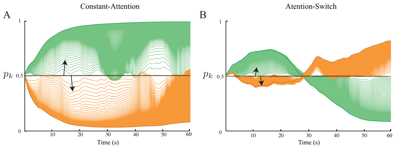
Figure 7: A step-wise illustration of the EM convergence. A) The output of the state-space decoder is plotted after each EM iteration for sample trials of attending to speaker 1 (green curves), and attending to speaker 2 (orange curves), in the Constant-Attention experiment. B) EM iterations are plotted for sample trials of the Attention-Switch experiment and for attention switches from speaker 1 to speaker 2 (green curves), and from speaker 2 to speaker 1 (orange curves). The iteration direction is shown by the arrows.
