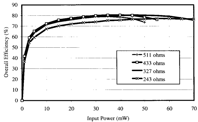
Fig. 12. Overall measured efficiency comparison of the 5.8-GHz rectenna with different resistive loads. The 327-Ω load gave the best match to the system with a VSWR of 1.29 at 50 mW of input RF power.
