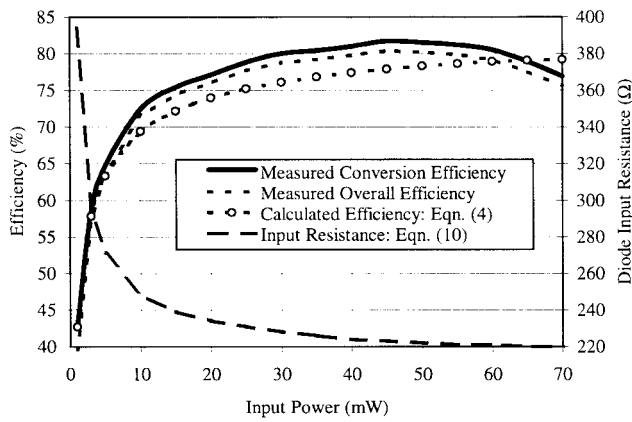
Fig. 10. Measured and calculated rectenna performance at 5.8 GHz with a 327-Ω load. A mismatch of the rectenna element with the system resulted in an efficiency decrease of 1% from the conversion to overall efficiency. A maximum conversion efficiency of 82% occurs at an input power of 50 mW. Also shown is the calculated diode input resistance as a function of input power.
